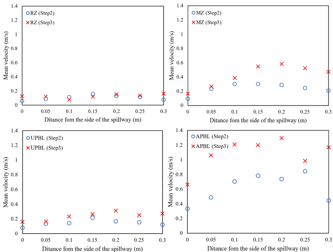
Fig. 5 Average velocity values on the areas formed on each step.
