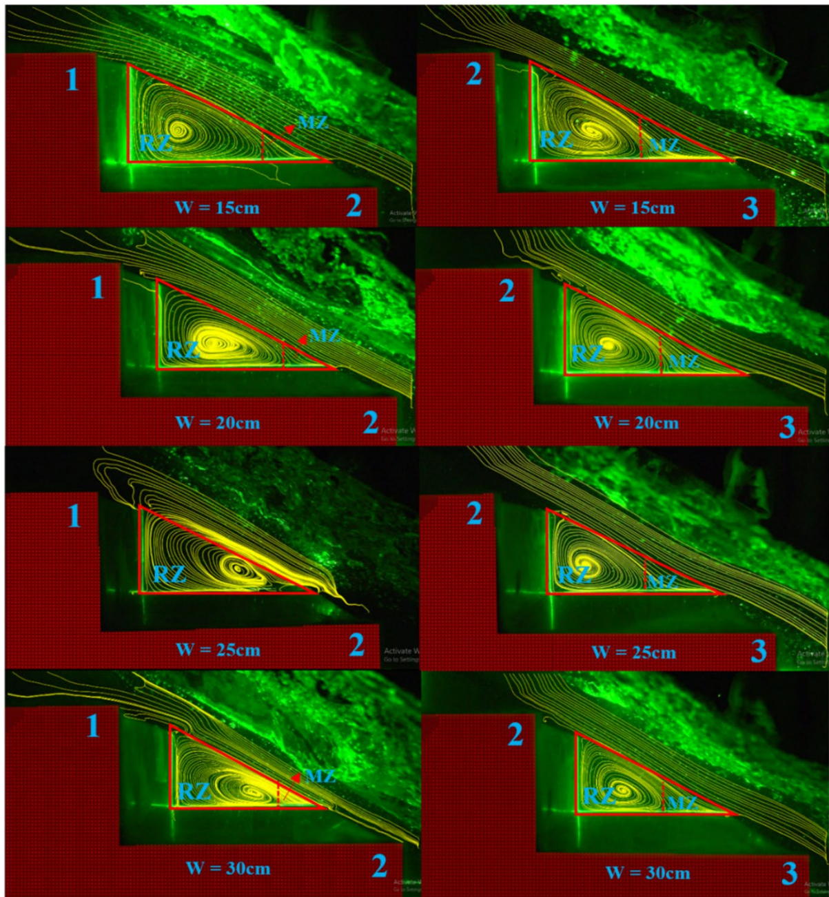
Fig. 3 The images of the zones developed under the pseudo-bottom line in the research's stepped spillway using PIV ( d_c/h = 1.09 ).
