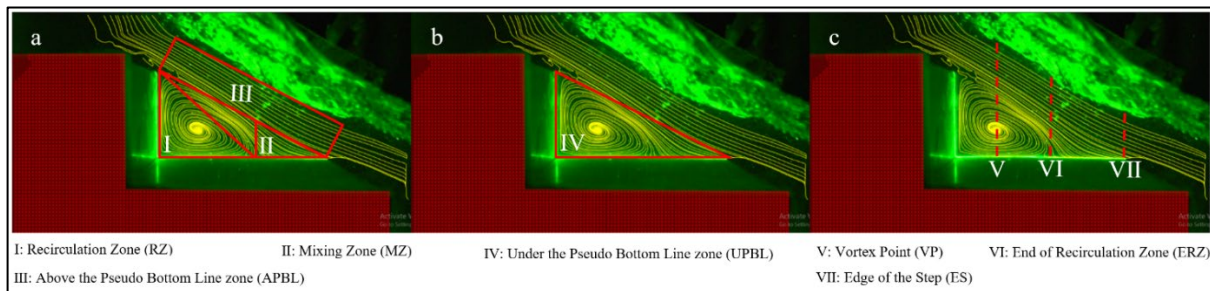
Fig. 4 Areas and points of collection of flow velocity on the steps.
