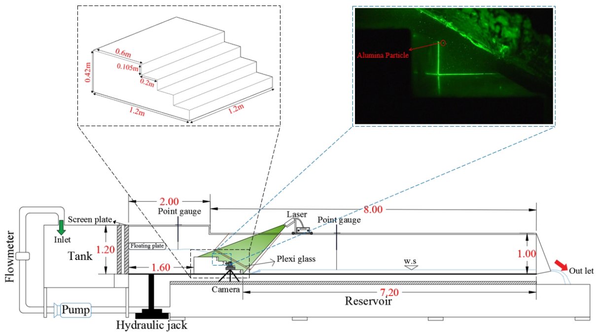
Fig. 2 The schematic view of the flume, the PIV system, and the spillway layout.
