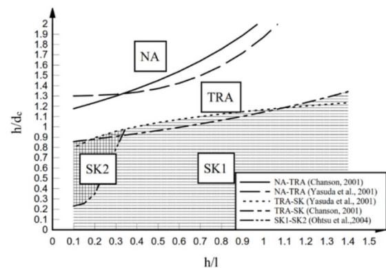
Fig. 1 Predicting the type of flow regime in stepped spillways (Image taken from Gonzalez & Chanson, 2006).
