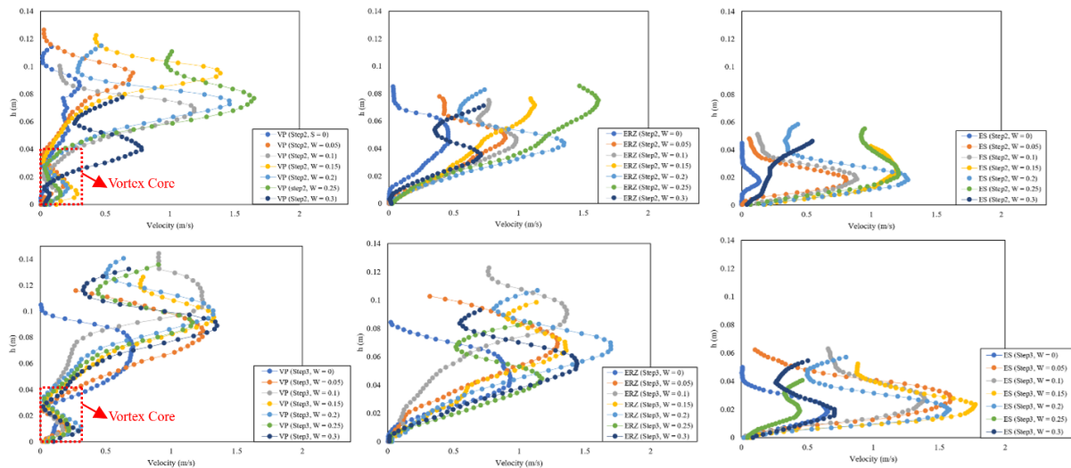
Fig. 6 Velocity profiles on the steps.
